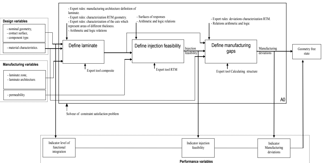
Fig. 4 Meta-model to determine industrialisation solutions (IDEF0 formalism).
