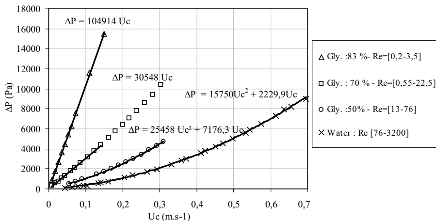
Fig. 14. Pressure drop as a function of the channel velocity for different liquids
