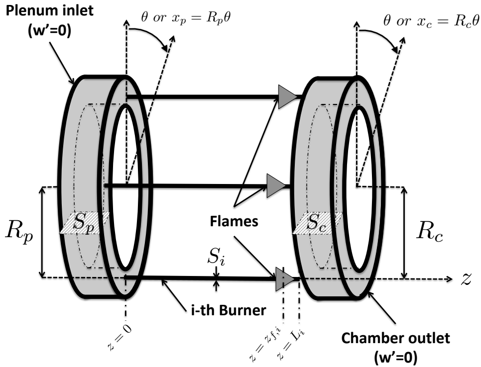
Figure 3: Network representation of the plenum, burners and chamber (PBC configuration)
