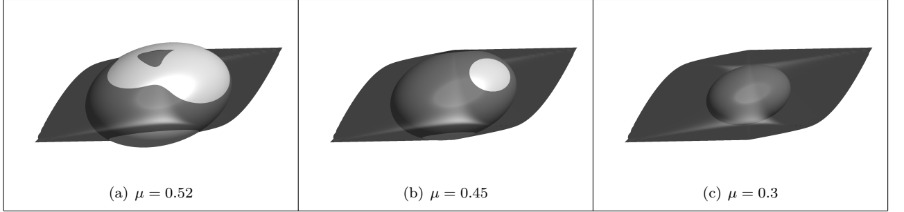
Figure 3: Examples of manifolds \mathcal{S}_\mu for different values of \mu . The unit ball \|\mathbf{s}\|_{\mathcal{S}} < 1 is in dark grey while the ellipsoid s_1^2 + 2s_2^2 + 3s_3^2 = \mu^2 is in light grey. The manifold \mathcal{S}_\mu is the part of the ellipsoid lying inside the unit ball. For small values of \mu , \mathcal{S}_\mu turns out to be merely the surface of the ellipsoid since it is entirely included in the unit ball.
