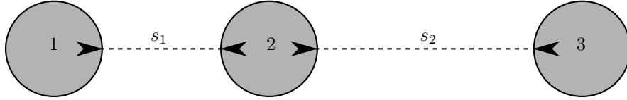
Figure 2: The linear 3-spheres swimmer is made of three spheres constrained to stay on a fixed line. The shape of the swimmer is determined by the lengths s_1 and s_2 of the bonds between spheres 1-2, and 2-3.
