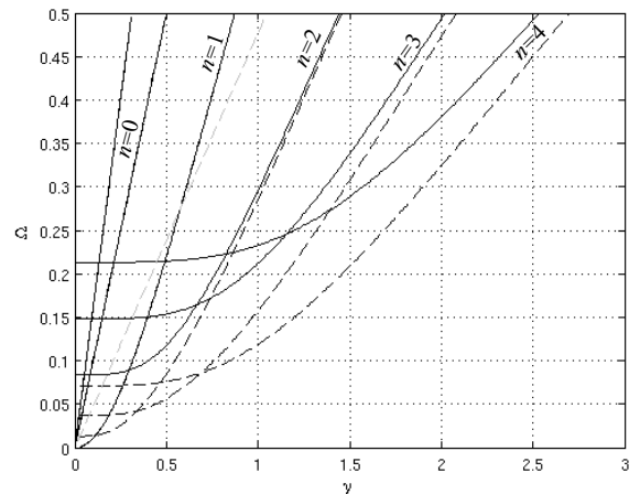
Fig.1 \Omega vs. \gamma for in vacuo elastic modes with pressurization (solid lines), without (dashed), and for the rigid wall acoustic mode (dashed grey).
