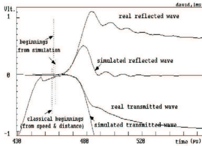
Fig. 14. Optimal choice of Young's modulus for transmitted and reflected waves.
