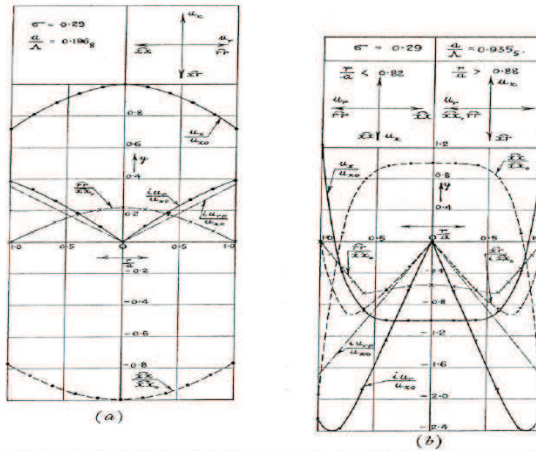
FIGURE 19. The variation of the displacements and the stresses over the cross-section of a bar of radius a . \frac{\partial u_x}{\partial x} = longitudinal stress; \frac{\partial u_r}{\partial r} = shearing stress; \frac{\partial u_r}{\partial r} = radial stress; u_x = longitudinal displacements; u_r = radial displacement; u_{r,p} = radial displacement in distortionless bar.
