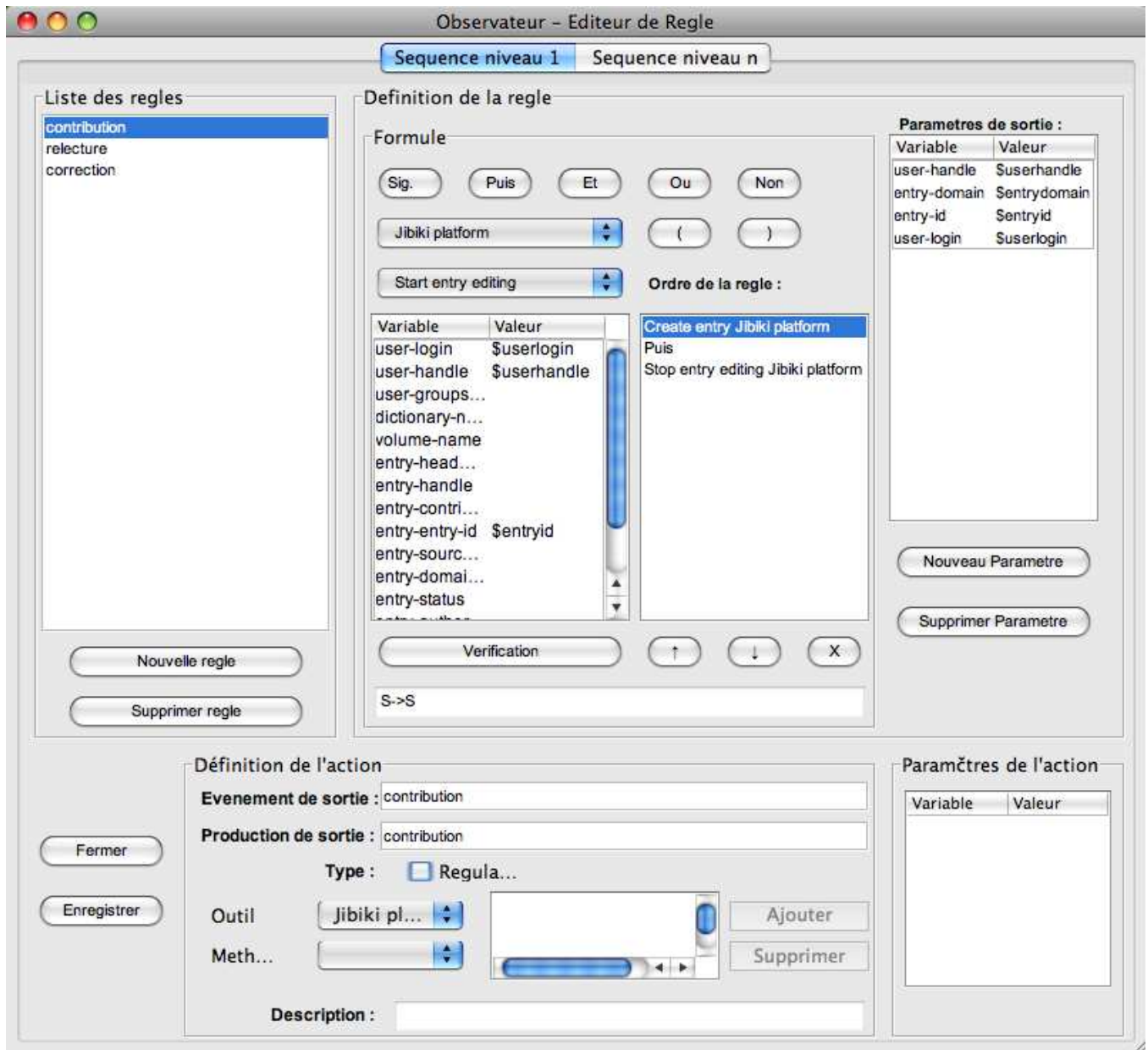
Fig. 4. Screenshot of the Rule Editor
