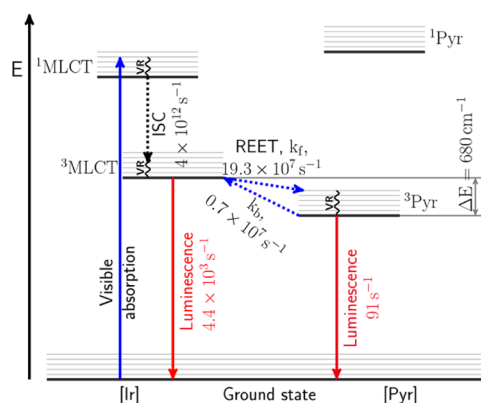
Figure 5. Jablonski diagram showing pertinent energy levels and kinetics of interchromophore energy transfer and luminescence of 2 . VR = vibrational relaxation, ISC = intersystem crossing, and REET = reversible electronic energy transfer. k_f and k_b correspond to the rates of forward and backward energy transfer, respectively.
