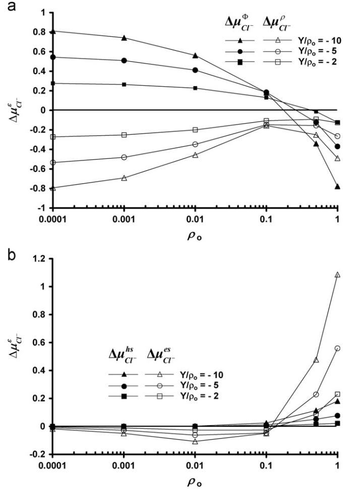
Fig. 5. Electrolyte: \text{CaCl}_2 . Species: \text{Cl}^- . Difference of each chemical potential contribution between the membrane centre and the left boundary vs. the salt density for several values of the membrane charge density ratio Y/\rho_o . (a) Density and electric potential contribution and (b) electrostatic and hard sphere contribution.
