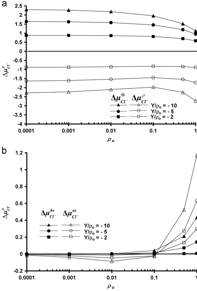
Fig. B4. Electrolyte: NaCl. Species: \text{Cl}^- . Difference of each chemical potential contribution between the membrane centre and the left boundary vs. the salt density for several values of the membrane charge density ratio Y/\rho_o . (a) Density and electric potential contribution and (b) electrostatic and hard sphere contribution.
