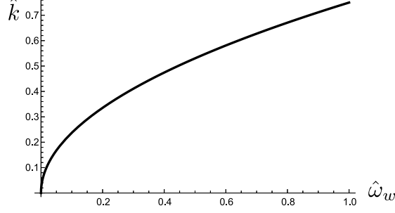
Figure 6: Variation of the dimensionless wave number \hat{k} = k(\alpha = \frac{\pi}{2}) \times \frac{\ell_w}{2\pi} according to the dimensionless frequency \hat{\omega}_w for macroscopic shear waves in the y direction. The dimensionless frequency is defined by \hat{\omega}_w = \omega \left(\frac{2\ell_w}{3\pi}\right)^2 \sqrt{\frac{\bar{\rho}_w}{E_w I_w}} \approx \frac{\omega}{\omega_{w1}} where \omega_{w1} is the circular frequency of the first bending mode of the floors with two fixed ends.
