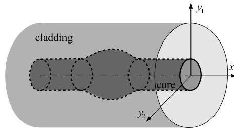
Figure 1: A locally perturbed uniform waveguide
