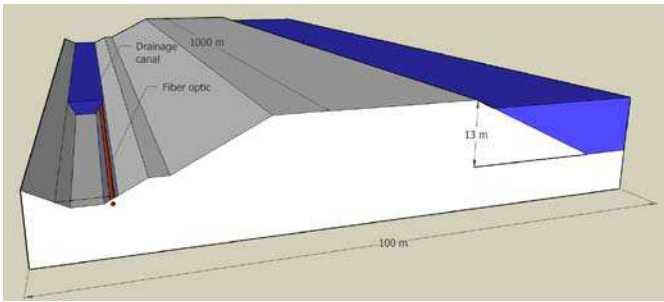
Figure 6: Representation of the global view of the instrumented dike of EDF.
