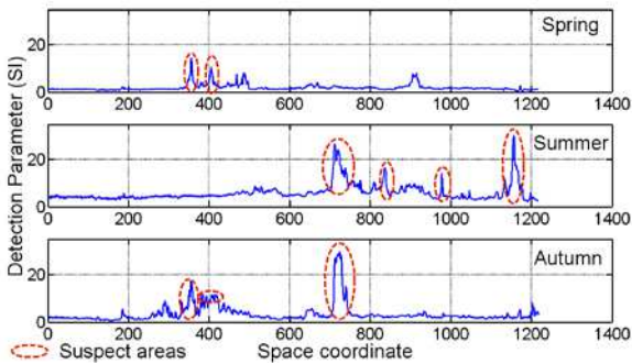
Figure 7: Results from the impulse method applied on the 2007 data.
