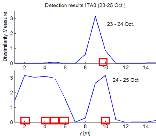
Figure 4: Analysis results for test #2 for the optical fiber placed at the downstream for last 2 days (23-25 October). Red rectangles represent leakages observed through visual inspections.
