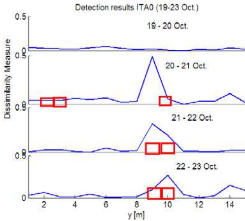
Figure 3: Analysis results (19-23 Oct. ) for test #2 for the optical fiber placed at the downstream. Red rectangles represent leakages observed through visual inspections.
