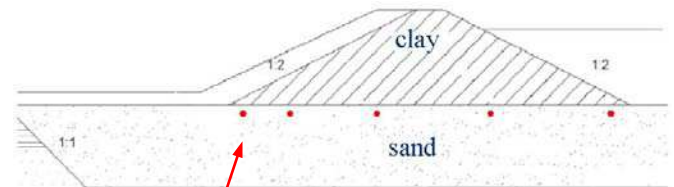
Figure 2: Cross-sectional view of the dike for a typical experimental phase showing the dike composition and placement of the optical fibers.
