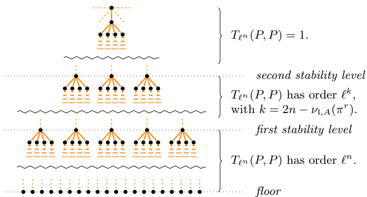
Fig. 4. Stability levels in the \mathfrak{l} -graph
