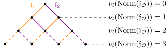
Fig. 2. The lattice of orders
