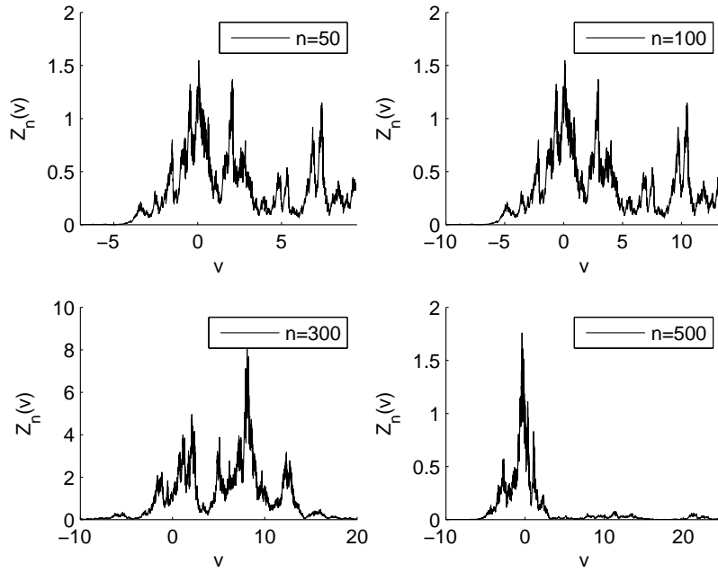
Fig. 1 Some realization of Z_{n,\vartheta_1}^*(v)
