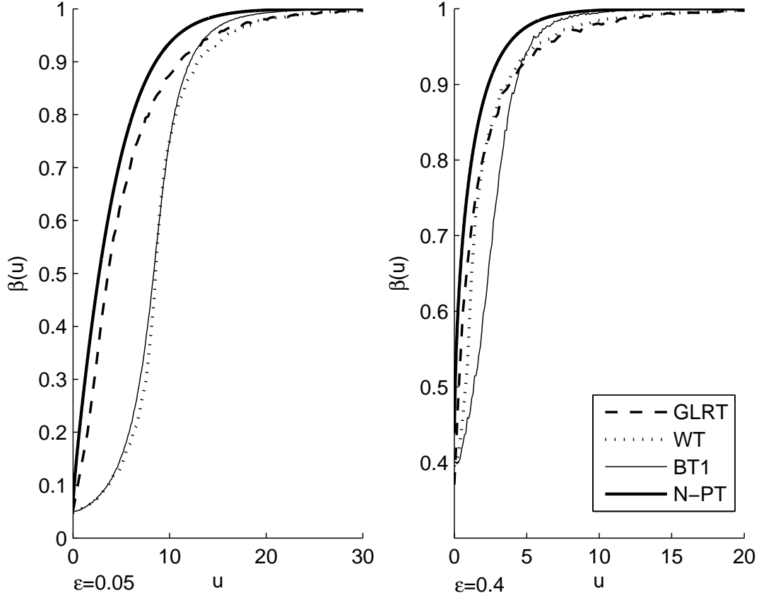
Figure 3: Comparison of limiting power functions for \varepsilon = 0.05 and \varepsilon = 0.4
