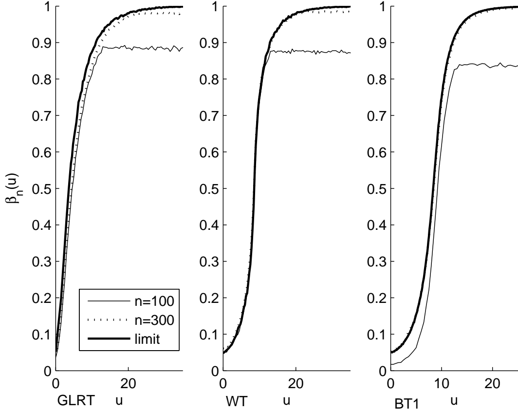
Figure 2: Power functions of GLRT, WT and BT1
