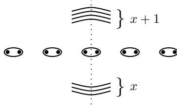
FIGURE 3. In the pignose diagram of \pi \in S_n if we draw a vertical line dividing the k th pignose in the middle, then the number of upper arcs intersecting with this line is equal to the number of lower arcs intersecting with this line plus 1.
