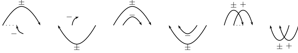
FIGURE 17. The list of configurations characterizing a crossing in the arrow diagram of a signed permutation.
