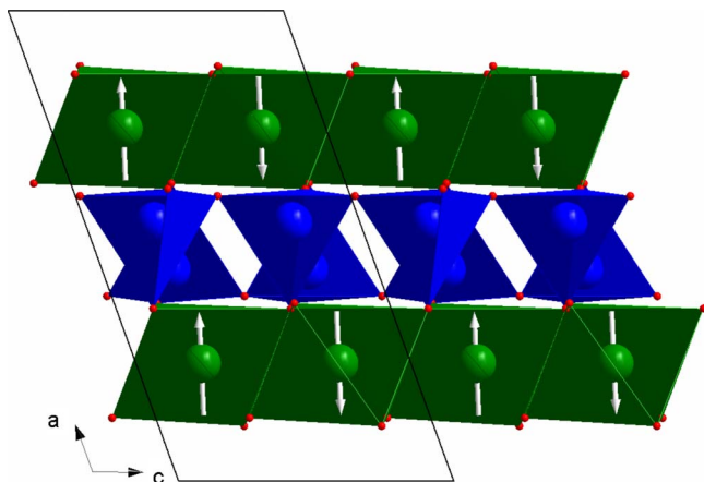
FIG. 4. (Color online) Magnetic structure of \text{LiCrSi}_2\text{O}_6 . The magnetic coupling between the \text{CrO}_6 chains is ferromagnetic while the magnetic coupling within the chains is antiferromagnetic.
