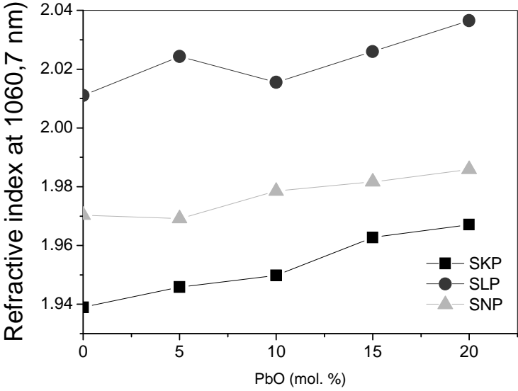
Figure 3: Variation of Refractive Index with PbO Molar Concentration.
