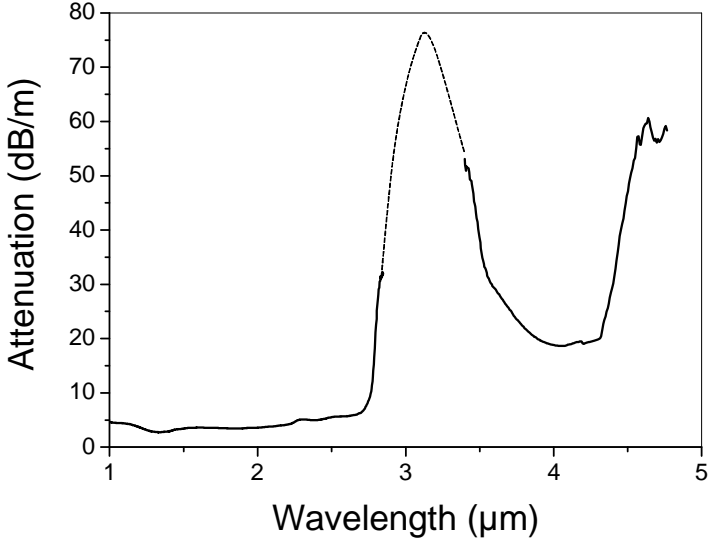
Figure 5: Attenuation curve of a Sb 2 O 3 based fiber, the dash curve concerns extrapolated points.
