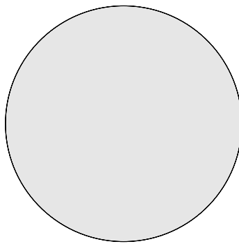
Figure 3: Circle : x^2 + y^2 = 1 , metric not unique
