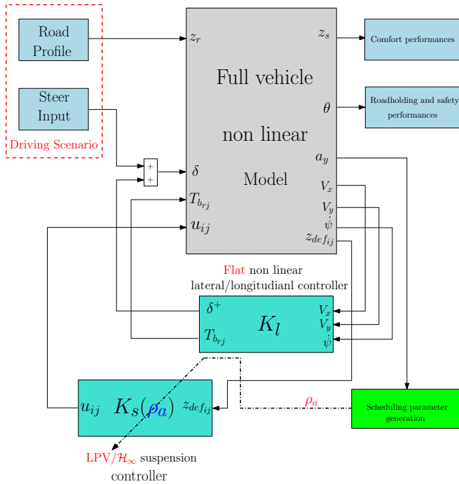
Fig. 1. Global chassis control integration strategy.
