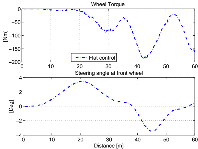
Fig. 4. Coupled longitudinal/lateral flat control signals
