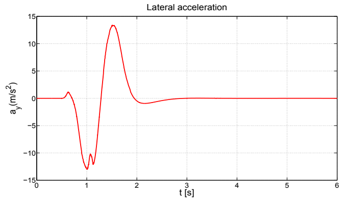
Fig. 7. Lateral acceleration
