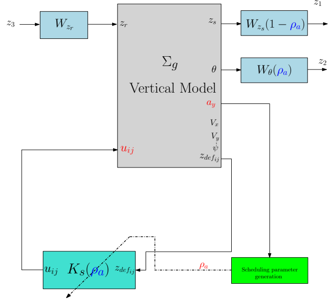
Fig. 3. General scheme of the LPV/ \mathcal{H}_\infty suspension control.
