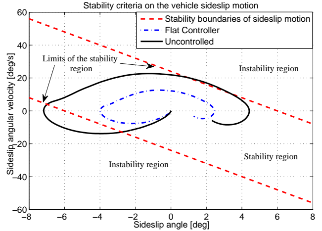
Fig. 6. Stability criteria of sideslip motion: controlled and uncontrolled vehicle models
