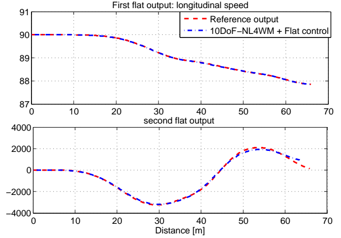
Fig. 5. Flat outputs: reference and controlled model
