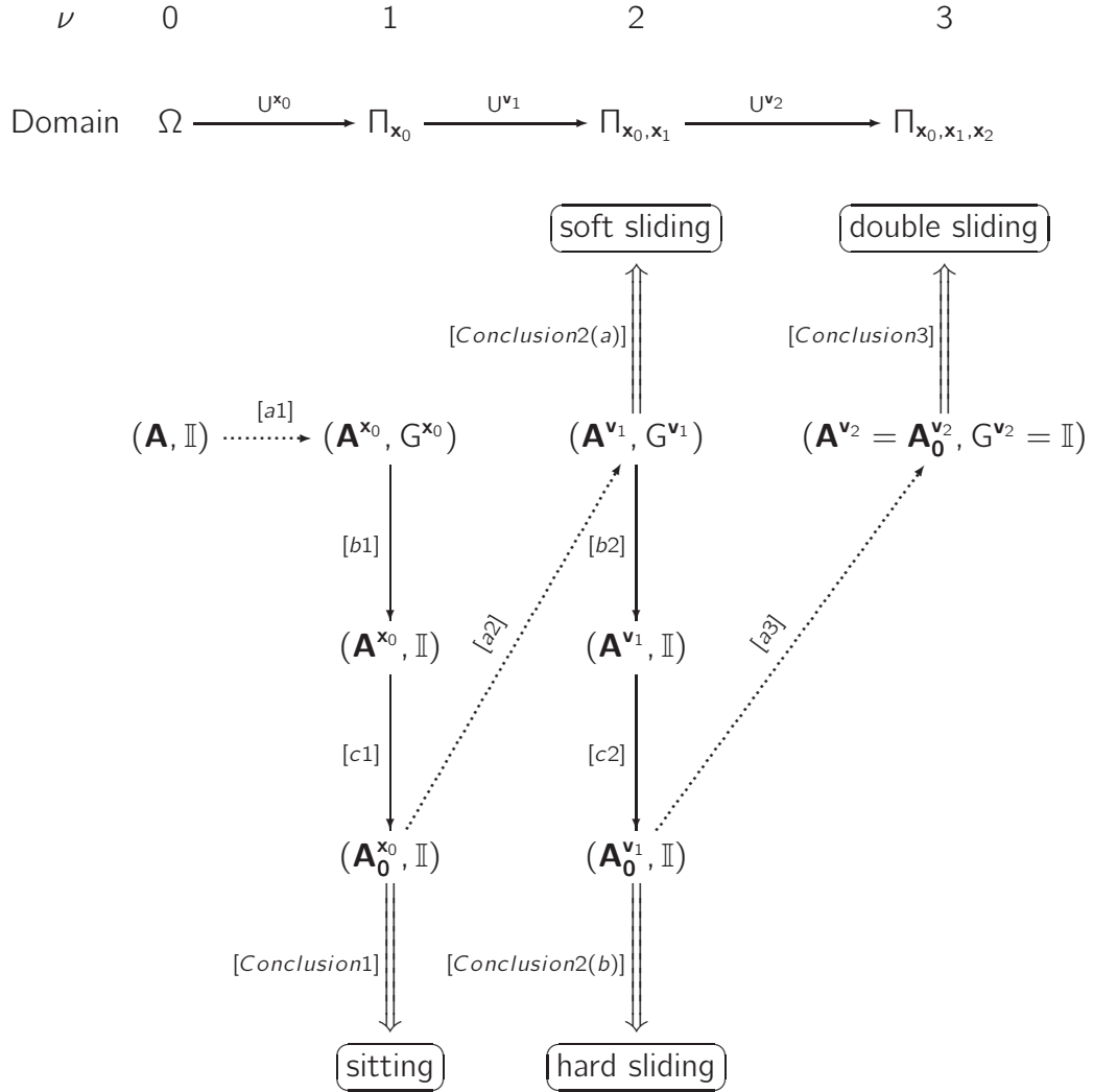
Figure 2. Construction of quasimodes
