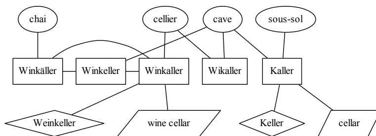
Figure 1: Simplified view of a subgraph. French words are in ellipses, Alsatian words in boxes, German words in diamonds and English words in parallelograms.
