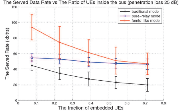
Fig. 5. the served data rate vs the fraction of embedded UEs (with 95% confidence interval)
