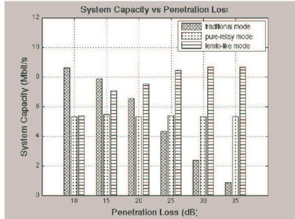
Fig. 6. System Capacity vs Penetration Loss
