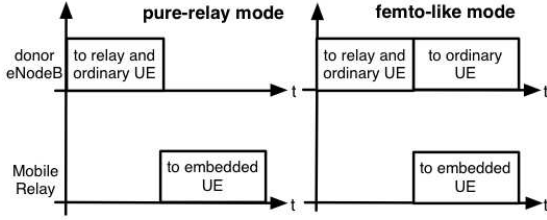
Fig. 3. The pure-relay mode vs The femto-like mode
