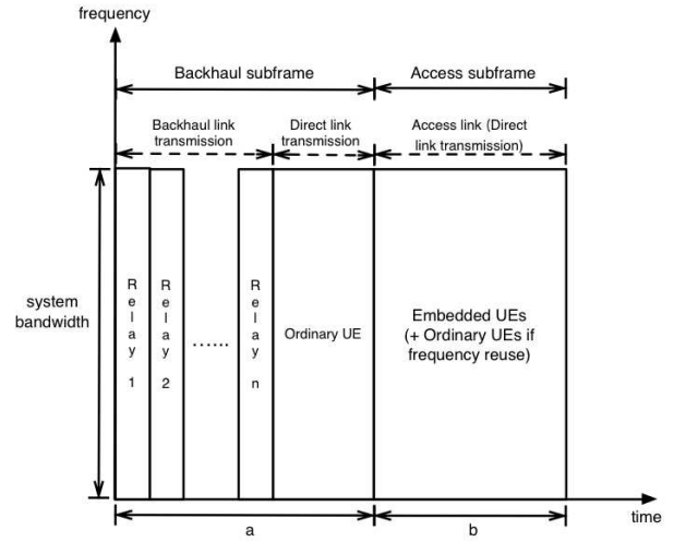
Fig. 4. Resource allocation in time domain
