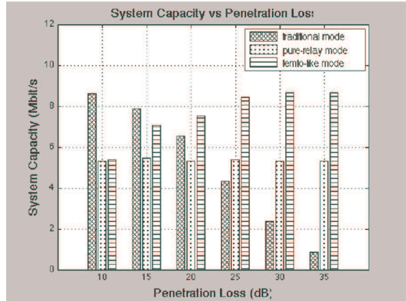
Fig. 6. System Capacity vs Penetration Loss
