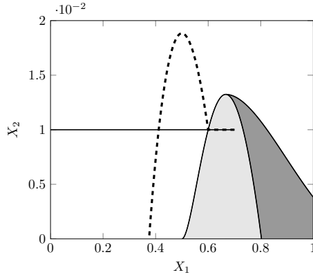
Figure 9: Two trajectories of an SIR evolution starts in X_0 = (0.7, 0.01) with \beta = 73 , \gamma = 36.5 , u_{max} = \infty , r_I = 1 and r_V = 1.5 . The solid curve corresponds to a trajectory with vaccination for all susceptible and the dashed trajectory with partial vaccination. The cost of the first strategy is 1.05 and the cost of the second strategy is 0.37.
