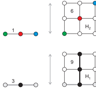
Figure 2: An illustration of the fact that the two types of geometric hyperplanes of S_{(2)} ( right ) can be regarded as blow-ups of the Veldkamp lines of S_{(1)} ( left ), or, vice versa , that a projection of a type two ( top right ) or type one ( bottom right ) hyperplane of S_{(2)} onto a line of S_{(2)} can be viewed, respectively, as the ordinary ( top left ) or an extraordinary ( bottom left ) Veldkamp line of S_{(1)} .
