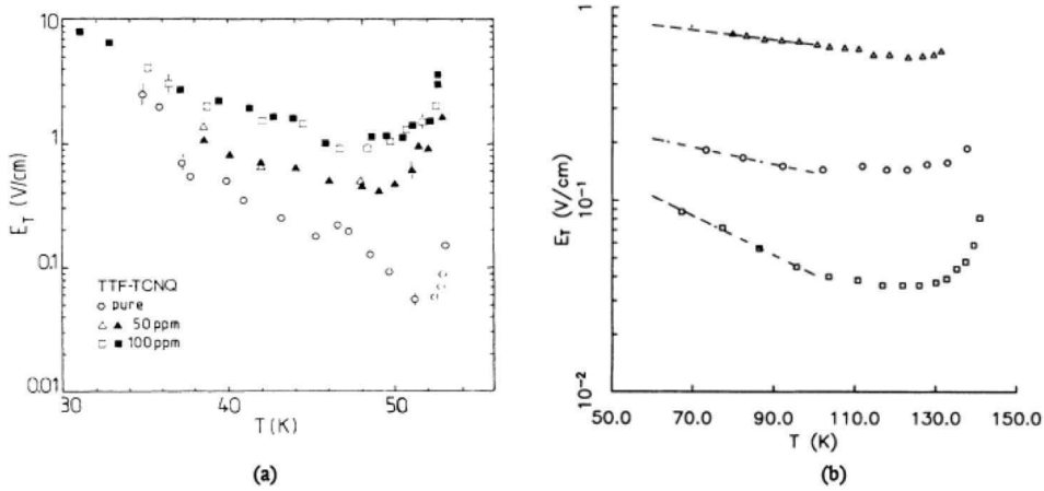
Figure 4.16. Variation of the threshold field E_T on log scale as a function of temperature. (a) For pure and electron-irradiation doped TTF-TCNQ crystals; (b) For \text{NbSe}_3 crystals containing different Ta concentrations. Dashed lines indicate the fit E_T \propto \exp(-T/T_0) (reprinted figure with permission from J. McCarten et al. , Physical Review B 46, p. 4456, 1992 [394]. Copyright (1992) by the American Physical Society).
