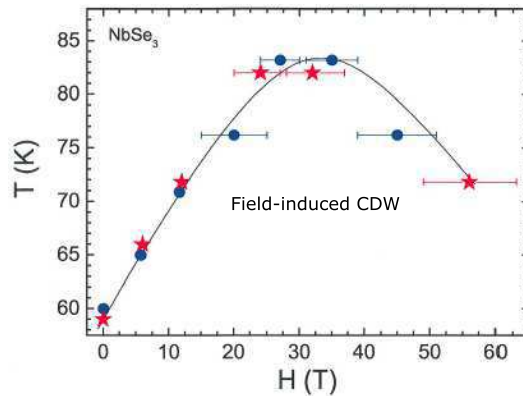
Figure 8.14. Phase diagram of the field-induced CDW state in \text{NbSe}_3 (reprinted figure with permission from Yu.I. Latyshev et al. , Physica B: Condensed Matter 404, p. 399, 2009 [801]. Copyright (2009) with permission from Elsevier).
