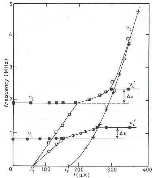
Figure 5.10. Variation of the fundamental narrow-band noise frequency \nu_\ell ( \circ , \square ) in a segment \ell ( 50 \mu\text{m} ) of a \text{NbSe}_3 crystal at 42 K as a function of the applied current i for two different constant currents above threshold in a neighbouring segment L ( 500 \mu\text{m} ) inducing a narrow-band noise frequency \nu_L ( \bullet , \blacksquare ) in L . The locking regime for each \nu_L is shown by half-black circles and half-black squares (reprinted figure with permission from M.-C. Saint-Lager et al. , Europhysics Letters 9, p. 585, 1989 [508]. Copyright (1989) from EDPSciences).
