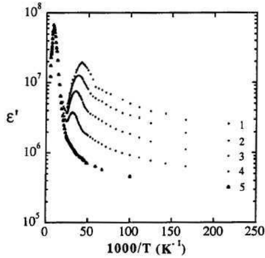
Figure 6.4. Dependence of the real part, \epsilon' , of the dielectric susceptibility of o-TaS 3 versus the inverse of temperature at frequencies (Hz): 1–11, 2–111, 3–1.1 10 3 , 4–10 4 , 5–10 5 (reprinted figure with permission from F.Ya. Nad and P. Monceau, Journal de Physique IV, Colloque C2 3, p. 343, 1993 [559]. Copyright (1993) from EdpSciences).
