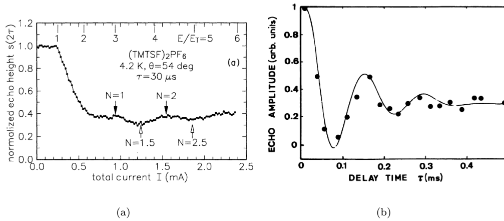
Figure 4.24. Variation of the amplitude of the spin echo (a) in (\text{TMTSF})_2\text{PF}_6 as a function of total current at 4.2 K (corresponding values of E/E_T are indicated on the top axis) with a pulse separation of 30 \mu\text{s} (reprinted figure with permission from W.G. Clark et al. , Physical Review B 49, p. 11895, 1994 [445]. Copyright (1994) by the American Physical Society), (b) in \text{R}_{0.3}\text{MoO}_3 at E/E_T = 20 and T = 49 \text{ K} as a function of the delay time \tau (reprinted figure with permission from P. Butaud et al. , Journal de Physique (France) 51, p. 59, 1990 [429]. Copyright (1990) from EdpSciences).
