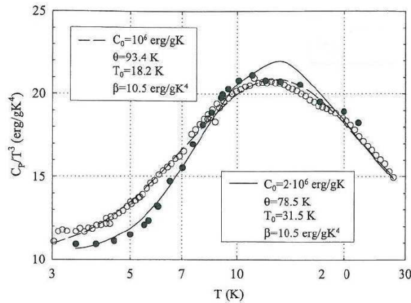
Figure 7.4. Specific heat in C_P/T^3 of a pure sample of K_{0.3}MoO_3 ( \circ ) and of a sample of a lower purity or structural quality ( \bullet ). Fits of the bump by the phason model (eq. (2.31)) are indicated by a continuous line for data ( \bullet ) and a dashed line for ( \circ ) with parameters reported in the insets (reprinted figure with permission from European Physical Journal B - Condensed Matter and Complex Systems 24, J. Odin et al. , p. 315, 2001 [644]. Copyright (2001) from Springer Science and Business media). Other data on the low temperature C_P of K_{0.3}MoO_3 were reported in [645] and [646].
