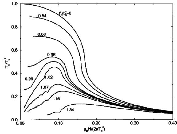
Figure 8.9. Phase diagram showing interplay between Pauli effect which tends to suppress the CDW and orbital effects which enhances the CDW for different values of the imperfect nesting parameter t'_b (reprinted figure with permission from D. Zanchi et al. , Physical Review B 53, p. 1240, 1996 [764]. Copyright (1996) by the American Physical Society).
