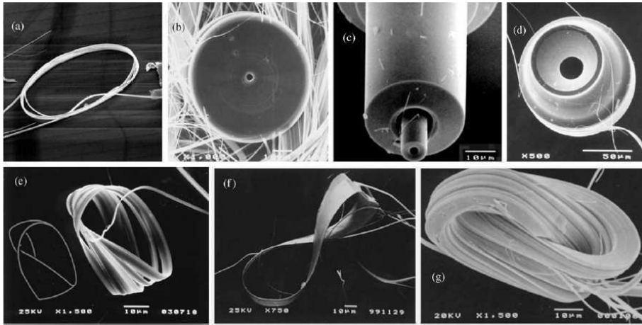
Figure 9.5. Scanning electron microscope images of \text{NbSe}_3 topological crystals with typical diameters between 10–200 \mu\text{m} : a) a basic ring or a thin short cylinder; b) a cylinder that grew radially; c) a cylinder grew longitudinally; d) concentric composite cylinders with a continuous or abrupt change in diameter; e) a Möbius strip with a \pi -twist; f) and g) a 2\pi twisted strip (reprinted figure with permission from T. Tsuneta and S. Tanda, Journal of Crystal Growth 264, p. 223, 2004 [824]. Copyright (2004) with permission from Elsevier).
