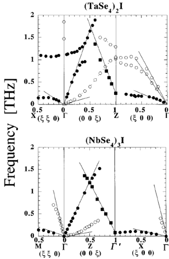
Figure 3.15. Phonon dispersion curves along high-symmetry directions from single crystal data at room temperature. Modes polarised along (normal to) the chain axis as shown as closed (open) circles: upper: (\text{TaSe}_4)_2\text{I} (reprinted figure with permission from J.E. Lorenzo et al. , Journal of Physics: Condensed Matter 10, p. 5039, 1998 [167]. Copyright (1998) by the Institute of Physics) and lower: (\text{NbSe}_4)_3\text{I} (reprinted figure with permission from Physica B 156-157, P. Monceau et al. , p. 20, 1989 [168]. Copyright (1989) with permission from Elsevier). Full lines correspond to the sound velocities taken from refs [169, 170] for (\text{TaSe}_4)_2\text{I} and ref. [169] for (\text{NbSe}_4)_3\text{I} .
