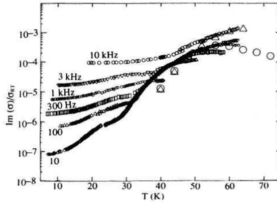
Figure 6.2. Temperature dependence of the imaginary part of the ac conductivity normalised to the room temperature value, \sigma_0 , of K_{0.3}MoO_3 at different frequencies. \circ ( \Delta ) are data at 1 kHz (10 kHz) from Cava et al. [541] (reprinted figure with permission from J. Yang and N.P. Ong, Physical Review B 44, p. 7912, 1991 [554]. Copyright (1991) by the American Physical Society).
