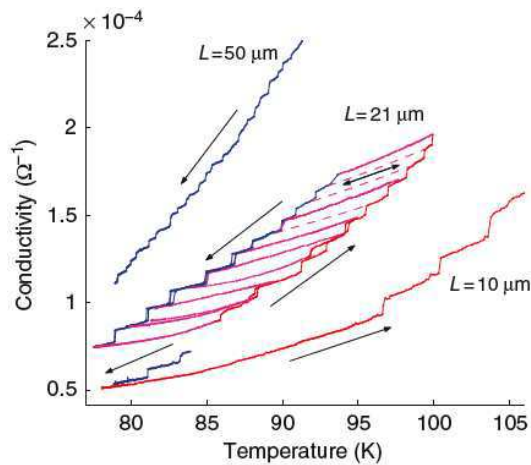
Figure 9.10. Temperature dependence of the conductivity of K_{0.3}MoO_3 samples with dimensions 21 \times 5 \times 0.3 \mu m^3 (central curve), 50 \times 7 \times 0.3 \mu m^3 (upper curve: \sigma is multiplied by 1.5), 10 \mu \times 5 \mu m^2 (lower curve: \sigma is divided by 15). The arrows indicate the direction of temperature sweep (reprinted figure with permission from S.G. Zybtssev et al. , Physica B: Condensed Matter 407, p. 1810, 2012 [473]. Copyright (2012) with permission from Elsevier).
