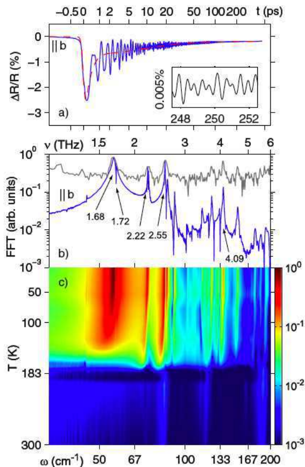
Figure 7.21. a) Transient change in reflectivity of \text{K}_{0.3}\text{MoO}_3 with \vec{E} \parallel \vec{b} at 10 K following photoexcitation with a 40 fs laser pulse. Dashed line is the fitted electronic transient. b) The FFT spectrum (amplitude) of the coherent parts of the signals, compared to recent Raman data (grey) [720]. c) T-dependence of the corresponding FFT spectrum in the range 1-6 THz (reprinted figure with permission from H. Schäfer et al. , Physical Review Letters 105, p. 066402, 2010 [718]. Copyright (2010) by the American Physical Society).
