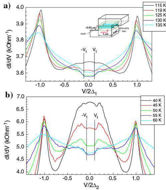
Figure 9.26. Tunnelling spectra dI/dV in NbSe_3 as a function of the voltage V normalised to the CDW gap 2\Delta at different T : a) upper CDW, b) lower CDW (reprinted figure with permission from Yu.I. Latyshev et al. , Physical Review Letters 96, p. 116402, 2006 [820]. Copyright (2006) by the American Physical Society).
