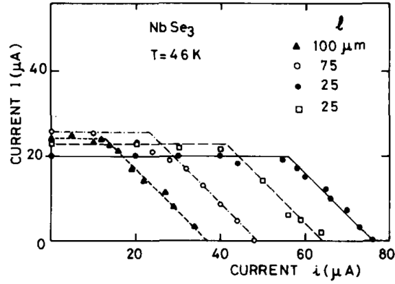
Figure 5.8. (I, i) diagram for depinning of a small segment of a NbSe 3 sample located between two electrodes apart of \ell for several values of \ell . The width of electrodes is 8 \mu\text{m} . I and i have the same meaning as in figure 5.7(a) (reprinted figure with permission from Physica B 143, P. Monceau et al. , p. 64, 1986 [506]. Copyright (1986) with permission from Elsevier).
