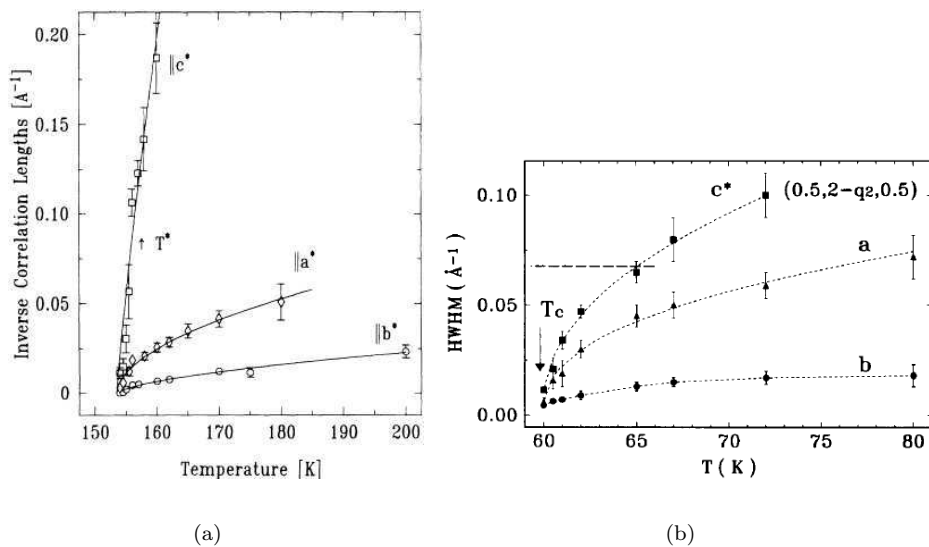
Figure 3.3. Temperature dependence of the inverse correlation lengths along three directions of NbSe 3 : a) through the Q_1 satellite reflection (reprinted figure with permission from A.H. Moudden et al. , Physical Review Letters 65, p. 223, 1990 [102]. Copyright (1990) by the American Physical Society); b) through the Q_2 satellite reflection (reprinted figure with permission from S. Rouzière et al. , Solid State Communications 97, p. 1073, 1996 [106]. Copyright (1996) with permission from Elsevier).
