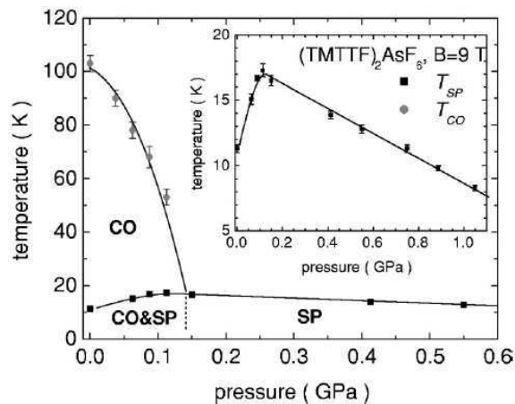
Figure 3.42. Phase diagram of (TMTTF) 2 AsF 6 under pressure showing coexistence between charge order and spin-Peierls ground states in the low pressure range (reprinted figure with permission from F. Zambrorsky et al. , Physical Review B 66, p. 081103(R), 2002 [257]. Copyright (2002) by the American Physical Society).
