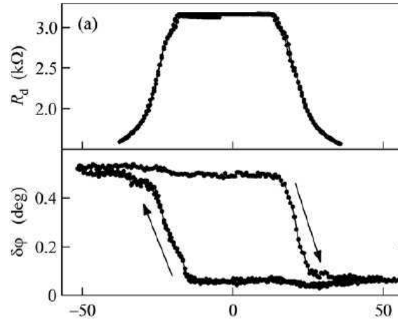
Figure 4.29. Variation of the rotation angle \delta\phi(I) and differential resistance R_d(I) measured simultaneously of a o\text{-TaS}_3 sample with one contact freely suspended (reprinted figure with permission from JETP Letters 92, S.G. Zybtssev et al. , p. 405, 2010 [473]. Copyright (2010) from Springer Science and Business media) at T = 121 K.
