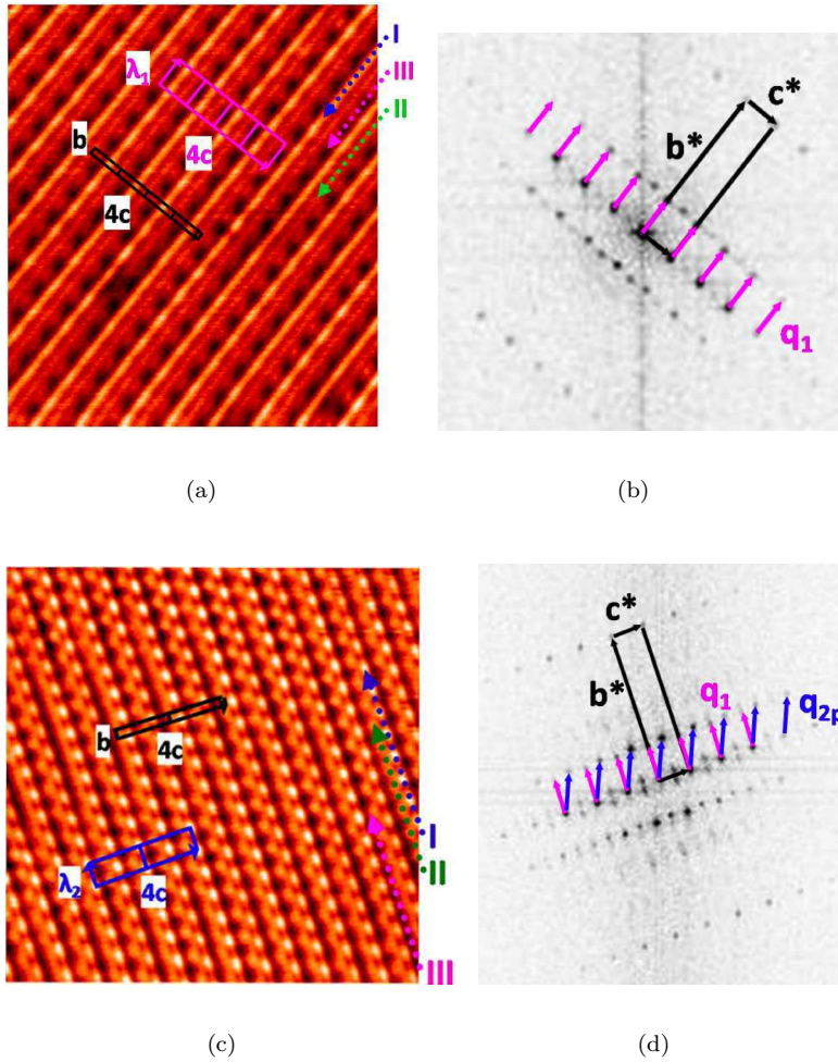
Figure 3.2. STM images of the (b, c) plane of in situ cleaved \text{NbSe}_3 . a) T = 77 K, scanned area 20 \times 20 \text{ nm}^2 . The unit cell is indicated together with the supercell of the Q_1 CDW. Three types of chains are identified, one of them carrying strong Q_1 CDW modulation is identified as chains III. CDW modulation forms bright maxima along the chains. V_{\text{bias}} = +100 mV, I = 1 nA. b) 2D Fourier transform of the STM image in a). The lattice Bragg spots, corresponding to b^* and c^* reciprocal vectors as indicated in black arrows, Q_1 CDW superlattice spots by purple vectors. c) T = 5 K, V_{\text{bias}} = +200 mV, I = 150 pA. The surface lattice unit cell and the Q_2 CDW surface superlattice are indicated by black and blue arrows ( \lambda_2 is the Q_2 period along the chain axis). d) 2D Fourier transform of the STM image shown in c). Q_1 and Q_2 CDW superlattice spots are indicated respectively by purple and blue arrows (reprinted figure with permission from C. Brun et al. , Physical Review B 80, p. 045423, 2009 [97]. Copyright (2009) by the American Physical Society).
