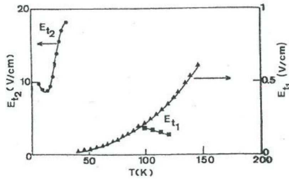
Figure 4.17. Variation of the threshold field E_T for K_{0.3}MoO_3 as a function of temperature (reprinted figure with permission from J. Dumas and C. Schlenker, International Journal of Modern Physics B 7, p. 4045, 1993 [326]. Copyright (1993) by World Scientific).
