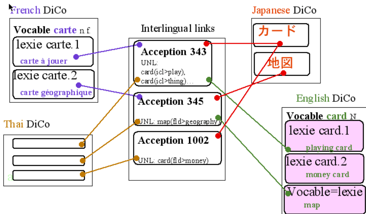
Figure 2. Lexical architecture of the papillon database
