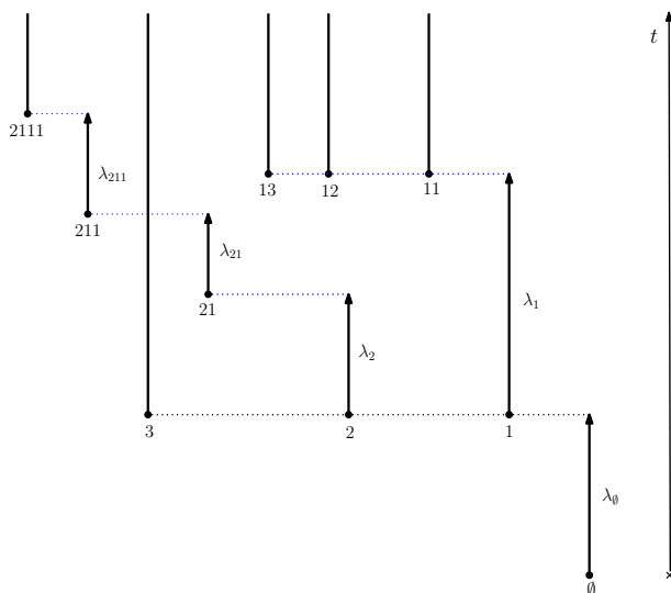
Figure 1 : Representation of a fragmentation as a process on \mathbb{U} .
