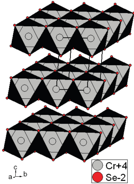
FIG. 1. (Color online) The schematic 3D structure of 1T - \text{CrSe}_2 . The selenium polyhedra centered on the metal ions are shown. The lines indicate the axes of the unit cell. This figure was generated by DIAMOND 2.1E 8 software.
