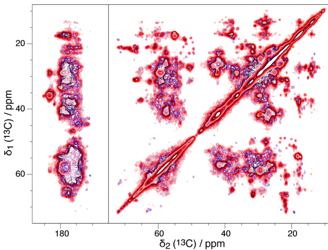
Figure S1. Overlay of the two-dimensional DARR spectra (50 ms mixing, 18 kHz MAS) of the 521 residue protein DnaB (molecular mass 59 kDa) microcrystalline (blue) and sedimented (red) DnaB sample.
