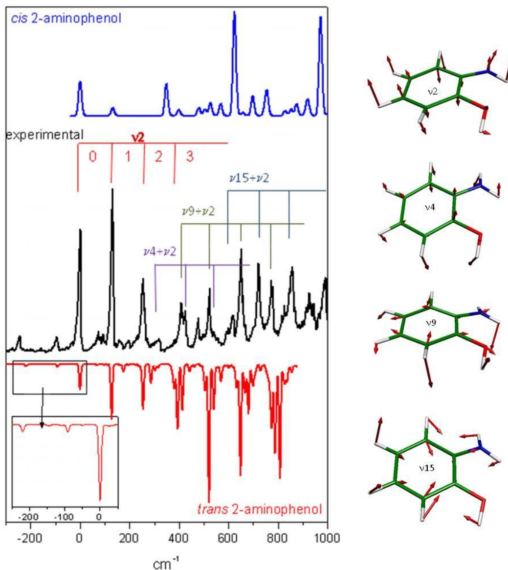
Figure 5: Left panel from top to bottom: simulated spectra using the ground and excited state frequencies calculated at the RI-CC2/aug-cc-pVDZ level for the cis isomer (blue) and for the trans isomer with a scaling factor of 0.82 (red) and experimental spectrum (black). The assignment of the vibrational bands is also shown on top of the experimental spectrum. Right panel: Scheme of the vibrational modes involved in the spectrum.
