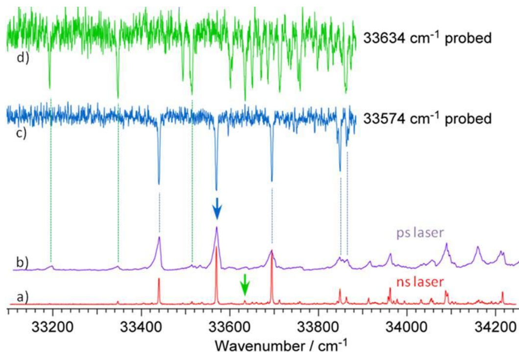
Figure 1: REMPI excitation spectrum recorded with a) ns laser with 0.08 \text{ cm}^{-1} resolution; b) ps lasers with 15 \text{ cm}^{-1} resolution. UV-UV hole burning spectrum pumping the band at c) 33574 \text{ cm}^{-1} (blue arrow) and d) the small band at 33634 \text{ cm}^{-1} (green arrow).
