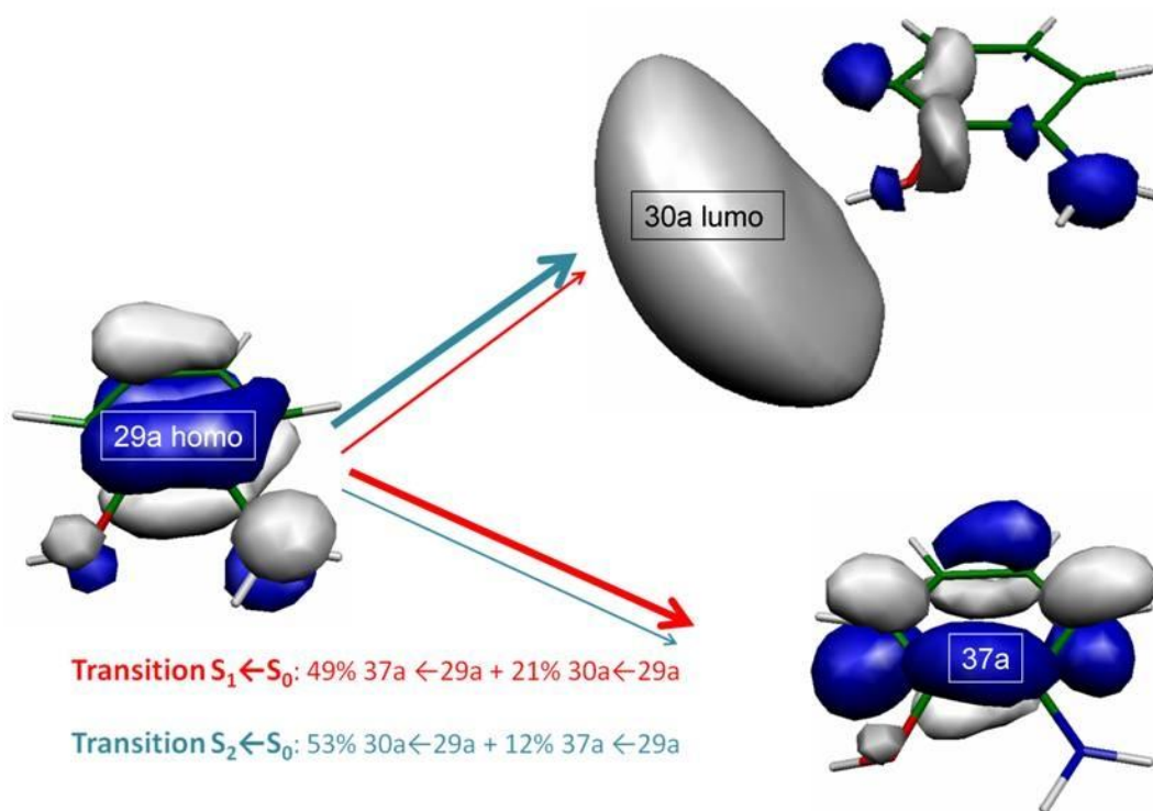
Figures 4: Orbitals involved in the S_1 \leftarrow S_0 and S_2 \leftarrow S_0 electronic transitions for the trans 2-aminophenol, calculated at the RICC2/aug-cc-pVDZ level.
