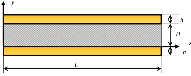
Fig. 1. Saturated porous medium of height H and length L bounded by two horizontal plates of height h . The upper and lower surfaces of the system are subject to a uniform heat flux. The vertical sidewalls are assumed to be perfectly insulated.
