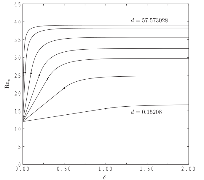
Fig. 4. Globally minimized neutral curves for Ra_c as functions of \delta for the following values of d : 57.573028, 19.16802, 5.67240, 2.71048, 1.67401, 0.78432 and 0.15208. These values have been chosen so that there exists a quartic minimum when \delta = 0.01, 0.03, 0.1, 0.2, 0.3, 0.5 and 1 , respectively; the locations of the quartic minima are shown by the bullet symbols. The neutral curves to the left of the symbols form straight lines in accordance with Eq. (15).
