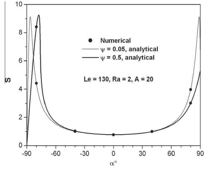
Fig. 3. Variation of the separation with the tilt angle for Le = 130 , Ra = 2 , A = 20 , and for \psi = 0.05, 0.5 .
