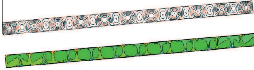
Fig. 8. Streamlines and isoconcentrations at the transition between the unicellular and the multicellular flows for Le = 100 , \psi = 0.1 , Ra = 42 , \alpha = 85^\circ and A = 20 .
