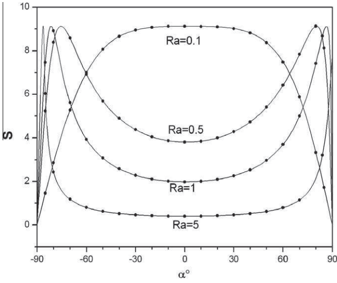
Fig. 2. Variation of the separation with the tilt angle for Le = 100 , \psi = 0.1 , A = 20 and Ra = 0.1, 0.5, 1, 5 . Solid curves represent the analytical results and the black dots the numerical results.
