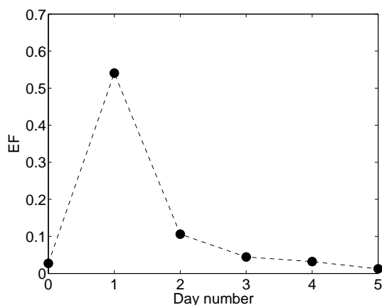
Fig. 5. Example of mean EF evolution before ( D0 ) and after ( D1 to D5 ) a rainfall which occurred at NG-fallow at the beginning of the monsoon.
