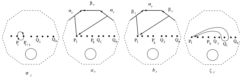
Figure 1: The generators \sigma_1, \dots, \sigma_{k-1}, a_1, b_1, \dots, a_g, b_g, \zeta_1, \dots, \zeta_n
