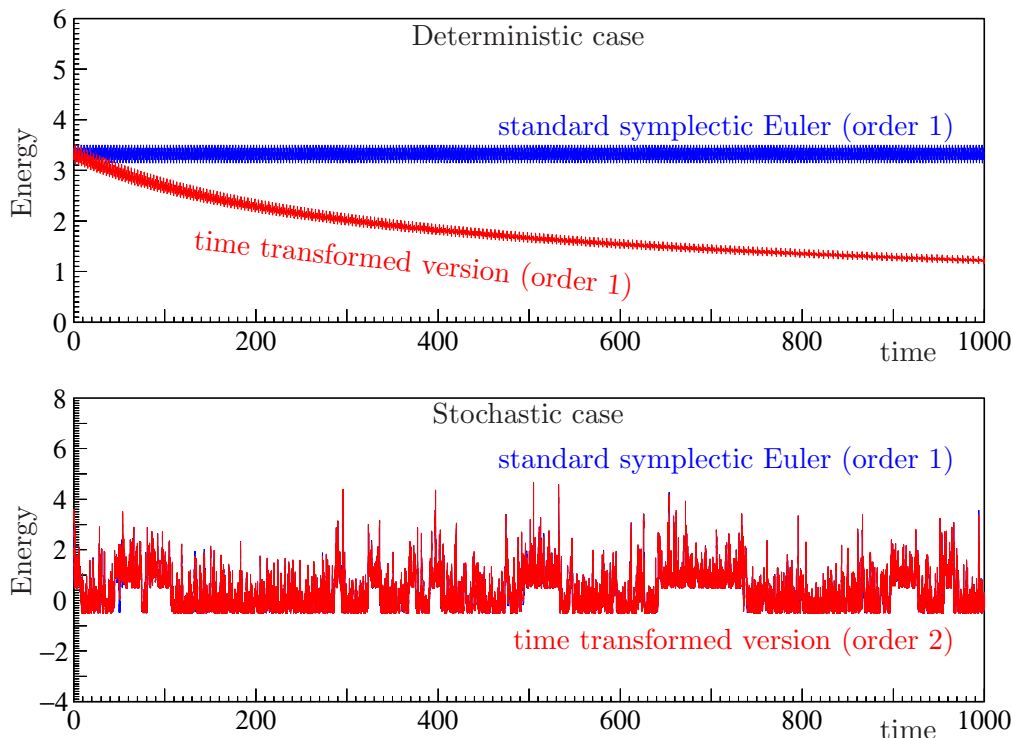
Figure 3: Evolution of the Hamiltonian energy (2) along time for the standard symplectic Euler method (34) and the time transformed version (35) (non symplectic) applied to (1) with V(q) = (1 - q^2)^2 - \frac{1}{2}q (quartic potential). Top picture: deterministic case ( \gamma = 0 ). Bottom picture: stochastic case ( \gamma = 4 ). Stepsize is h = 0.02 and \beta = 2 .
