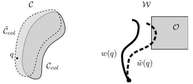
Fig. 2. Correspondance between approximation of the rod geometry \tilde{w}(q) in the workspace \mathcal{W} (right) and approximation of the environment colliding space \tilde{\mathcal{C}}_{col} in the configuration space \mathcal{C} (left). In this case, the approximation of the geometry induces a false invalid configuration detection.
