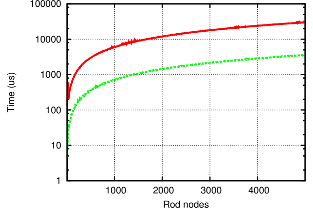
Fig. 1. Log scale computation time of the DGM (red) and its first order approximation (green).
