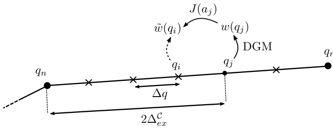
Fig. 3. Local path validation using DGM Jacobian approximation. The approximation of the geometry \tilde{w}(q_i) is obtained using the geometry w(q_j) of the closest configuration q_j having exact geometry. Crosses (resp. dots) represent configurations where the DGM will be approximated (resp. fully computed).
