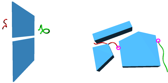
Fig. 5. The two toy scenarios used for benchmarks: crack (left) and backward (right). Start (resp. goal) configurations of the rod are represented in green (resp. red). Note the head of cable has been marked with a magenta circle on the Benchmark scenario to emphasize solution path could not be obtained with a point-like robot.
