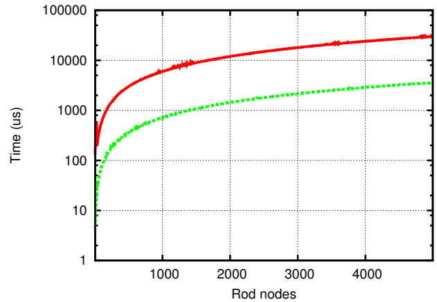
Fig. 1. Log scale computation time of the DGM (red) and its first order approximation (green).
