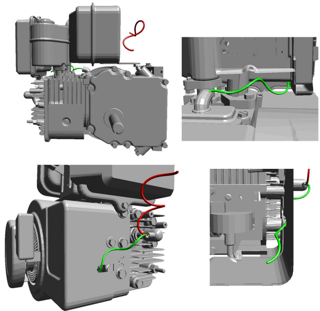
Fig. 6. Two industrial cases of disassembling for a free-flying cable (top) and a fixed base cable (bottom). The cable has to get out from a highly constrained start configuration (in green) to a low constrained configuration (in red). Closer views on the start configuration are represented on the right for each scenario.
