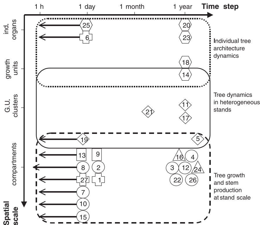
Figure 3. Schematic location of each tree growth model reviewed in a space-time domain. Each symbol corresponds to a major model objective (○: simulation of individual tree architecture dynamics; ○: prediction of tree growth and stem production; △: prediction of stem profile; ◻: research tool; ◇: simulation of tree dynamics in forest stands; ◻: prediction of fruit yield at tree level). Arrows indicate the range of time steps used for the different processes represented. Numbers in symbols refer to models (1: [100]; 2: [1]; 3: [132]; 4: [73]; 5: [97]; 6: [102]; 7: [128]; 8: [138]; 9: [141]; 10: [139]; 11: [120]; 12: [142]; 13: [40]; 14: [123]; 15: [147]; 16: [23]; 17: [41]; 18: [51]; 19: [71]; 20: [93]; 21: [144]; 22: [9]; 23: [103]; 24: [24]; 25: [4]; 26: [75]; 27: [29]).
