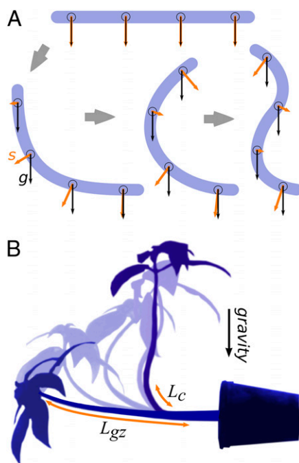
Fig. 1. Shoot gravitropism beyond the sine law. (A) Diagrams of a stem responding to gravity according to the sine law. Sensing and curving are distributed over the entire length of the stem. The orange arrows indicate the component of the gravity vector ( g ) that serves as the effective bending stimulus ( s ). The stem repeatedly overshoots the vertical because the basal part of the stem is still receiving a strong stimulus and is therefore actively curving even as the apical part approaches the vertical. (B) The gravitropic response of Impatiens glandulifera sketched from Pfeffer’s original photographs. This plant is a prime example of a gravitropic response with a large bending number ( B \sim 9 ). It overshoots the vertical twice, thus forming first a “C” and then a “S” shape, but ultimately converges on a stable configuration whereby a large section of the stem is straight. The first two time points of the response highlight the development of curvature over the extensive growth zone ( L_{gz} ), whereas the last time point shows the curvature converging ultimately to a much shorter length scale ( L_c ). The rapid convergence to an erect configuration is indicative of the stabilizing effect of autotropic straightening in gravitropic responses.
