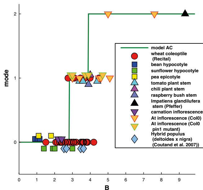
Fig. 6. Mode number M plotted against bending number B = L_{gz}/L_c for individual plants ( N = 67 ). The green line shows the same plot for the AC model.
