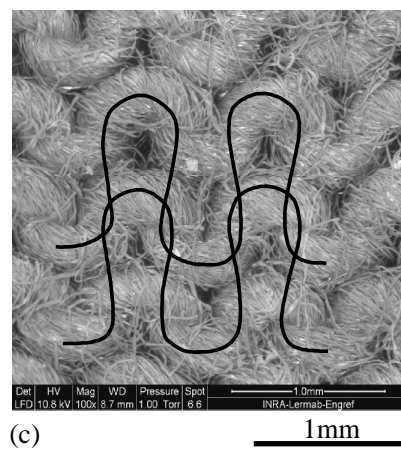
Fig. 4: Structure of the Jersey knitting cotton ready-to-wear clothing: Image obtained by x-ray attenuation (a). Micrographs obtained by electronic microscopy (ESEM). Front face (b) and back face (c). (LERMAB by F. Huber)
