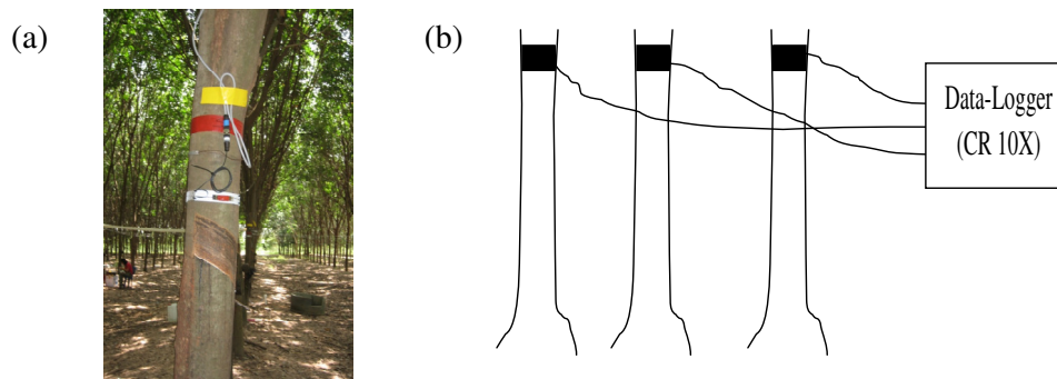
Fig 1. Photograph of (a) electronic dendrometer sensor for measuring micro-change of trunk girth variations and setting at a height of 180 cm above the ground level. Each dendrometer sensor attached to each of the three mature rubber trees. The three dendrometer sensors (b) were connected to a data logger (model CR 10X).
