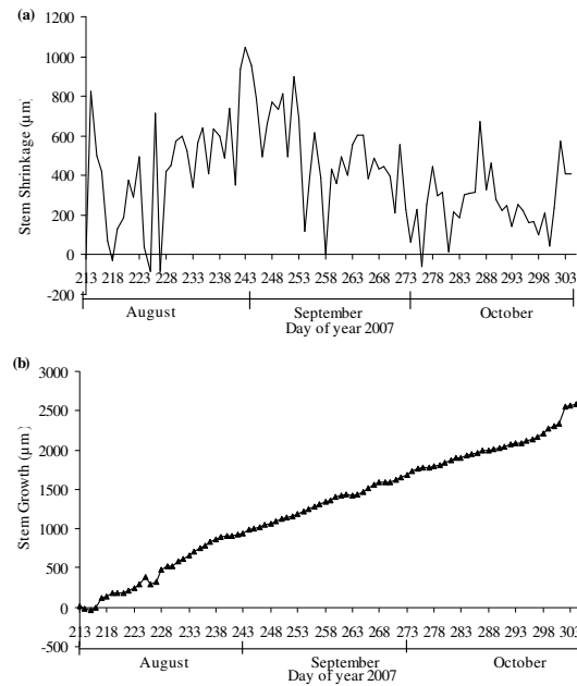
Fig 3. Diurnal course of (a) maximum daily trunk shrinkage (MDS) and (b) trunk circumference growth (expansion shown as positive values; contraction as negative values) in mature rubber trees measured at 180 cm above the ground level, 1 August - 31 October, 2007. Each data point represents the mean daily change in MDS and growth of three mature rubber trees under non-limiting soil moisture.
