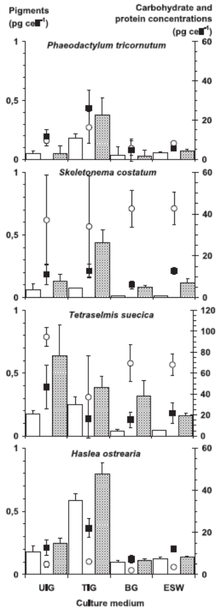
Fig. 2. Carotenoid ( \square ), chlorophyll a and pheopigment ( \boxtimes ), carbohydrate ( \circ ) and protein ( \blacksquare ) contents of cultures ( \text{pg cell}^{-1} ) grown in Untreated Ifremer Groundwater (UIG), Treated Ifremer Groundwater (TIG), Bouin Groundwater (BG) and Enriched SeaWater (ESW). Mean \pm confidence interval.
