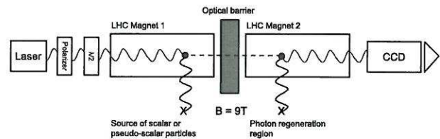
Figure 1: Experimental setup for Photon regeneration experiment
