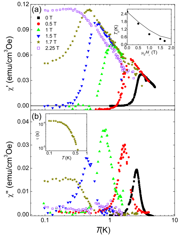
FIG. 1: (Color online) \chi' (a) and \chi'' (b) measured at \omega/2\pi = 333 \text{ Hz} and different H_\perp . The inset in (a) shows the shift of \chi'' maxima with increasing H_\perp . The solid line shows theoretical predictions for quantum spin-phonon relaxation that follow from Pauli's master equation as described in [28]. The inset in (b) shows the magnetic relaxation time at \mu_0 H_\perp = 1.7 \text{ T} .
