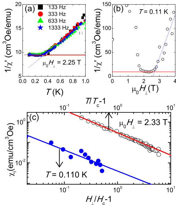
FIG. 2: (Color online). (a) and (b): 1/\chi' measured at \mu_0 H_\perp = 2.25 T as a function of T and at T = 0.110 K as a function of H_\perp , respectively. The crossovers between the "Curie-Weiss" law, observed at either high T or high H_\perp (dotted blue lines), and the ferromagnetic limit 1/\chi' = N (solid red lines) give T_c (= 0.34(1)\text{K}) and \mu_0 H_c (= 2.65(5) T), respectively. (c) Log-log plot of demagnetization-corrected \chi'_i vs the reduced temperature (for \mu_0 H_\perp = 2.33 T with T_c = 0.31 K, \circ ) and field (at T = 0.110 K with \mu_0 H_c = 2.65 T, \bullet ). The linear fits give critical exponents \gamma_{cl} \simeq 1.1(1) and \gamma_{qu} \simeq 1.0(1) .
