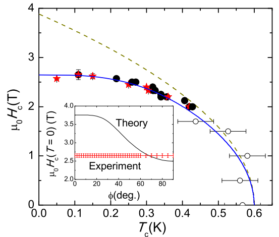
FIG. 3: (Color online) H_c - T_c phase diagram determined from the linear extrapolation of 1/\chi' to 1/\chi_{\max} , as shown in Figs. 2a and b. \bullet and \circ correspond to T_c > T_b and T_c < T_b , respectively; \star , data determined from susceptibility scaling plots, as those shown in Fig. 2(c). Solid line, quantum mean-field calculation of the phase boundary using Eq. (4); dashed line, classical phase diagram, derived from MC simulations. Inset: zero-temperature critical field vs angle \phi . The horizontal line represents the experimental H_c(T_c = 0) .
