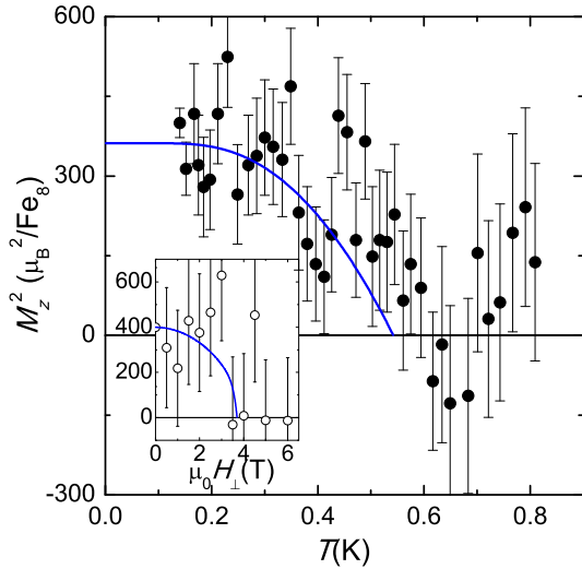
FIG. 4: (Color online) Squared longitudinal magnetization of a \text{Fe}_8 crystal determined from neutron diffraction intensities measured at \mu_0 H_{\perp} = 1.5 T. The inset shows data measured at T = 0.14 K as a function of H_{\perp} . The lines are mean-field calculations using Eq. (4) with \phi = 0 .
