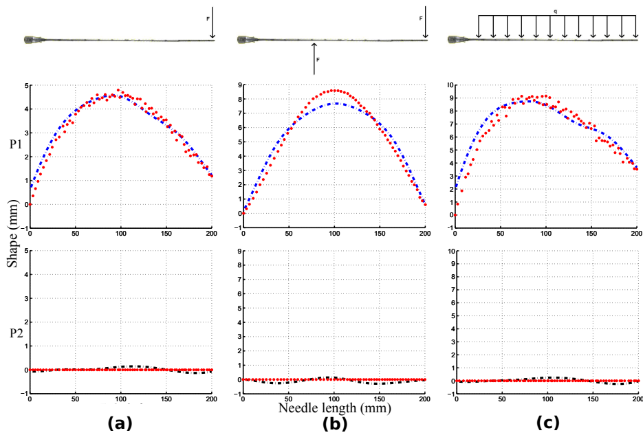
Figure 13: Reconstruction of TH needles deflections. a ) Modeling in the case of concentrated radial forces in planes P1 and P2, b ) Modeling in the case of two concentrated radial forces in planes P1 and P2, c ) Reconstruction with constant force distribution in planes P1 and P2. The dots represent the segmented needle trajectory and the dashed lines represent the needle trajectory reconstructed using the force basis.
