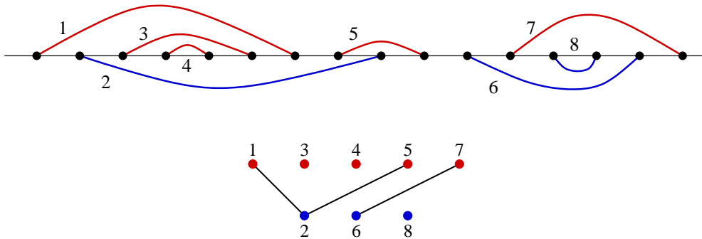
Fig. 3: The arch system associated with the operation sequence I_1 I_2 I_1 I_1 O_1 O_1 O_1 I_1 O_2 O_1 I_2 I_1 I_2 O_2 O_2 O_1 , and the associated graph. The arches are labelled using the left-to-right order of their left endpoint. This arch system has five connected components, and one left-right pair (between arches 2 and 5). The output permutation is 43125867.
