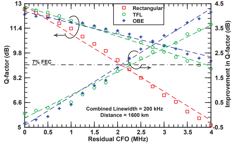
Fig. 4. Impact of utilizing rectangular, TFL and OBE pulse shapes under varying residual CFOs at transmission distance of 1600 km.
