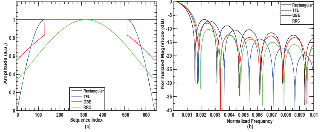
Fig. 1. Rectangular (black), TFL (blue), OBE (red) and RRC (green, \alpha = 1 ) depiction of (a) impulse response and (b) frequency response. Rectangular has very high energy sidelobes. TFL pulse shape exhibits better localization in time and frequency than OBE. The difference between TFL and OBE is that TFL has higher sidelobe energy and quick energy decay; on the other hand OBE has lower sidelobe energy and slow energy decay. RRC shows good sidelobe energy, however it introduces high inter-symbol interference.
